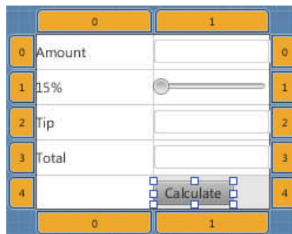
Figura 25.13 | GridPane preenchido com controles do Tip Calculator.
